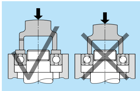
Fig. 15.13 Simultaneous press-fitting
