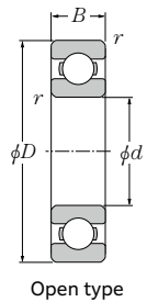
Open type
