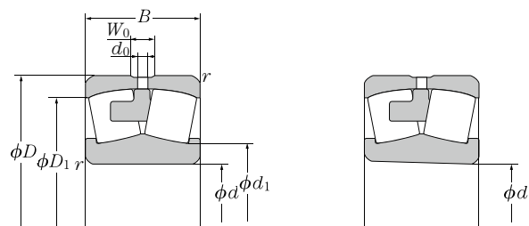
Cylindrical bore
