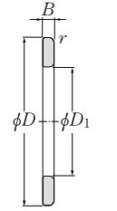
GS type raceway (Outer ring)
