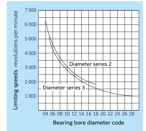
Fig. 1 Allowable speed of ball bearings for units
