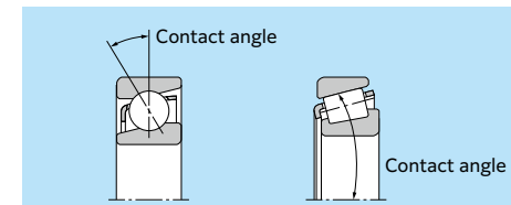
Fig. 1.3 Contact angle
